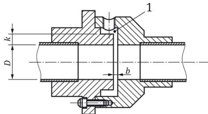
Figure G.1 — Example of drilled hole type of pressure tapping with ring chamber, suitable for small/medium diameter test sections
