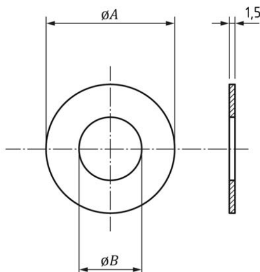
Figure H.12 — Gasket of a wafer type disturbance generator, with dimensions as set out in Table H.8
