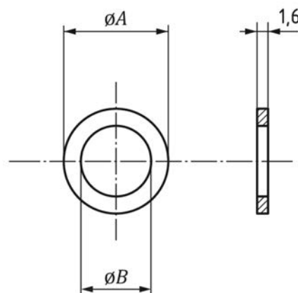
Figure H.7 — Gasket for a threaded type disturbance generator, with dimensions as set out in Table H.5
