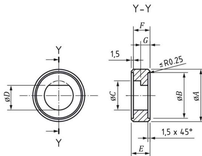
Figure H.6 — Flow disturber for a threaded type disturbance generator, with dimensions as set out in Table H.4
