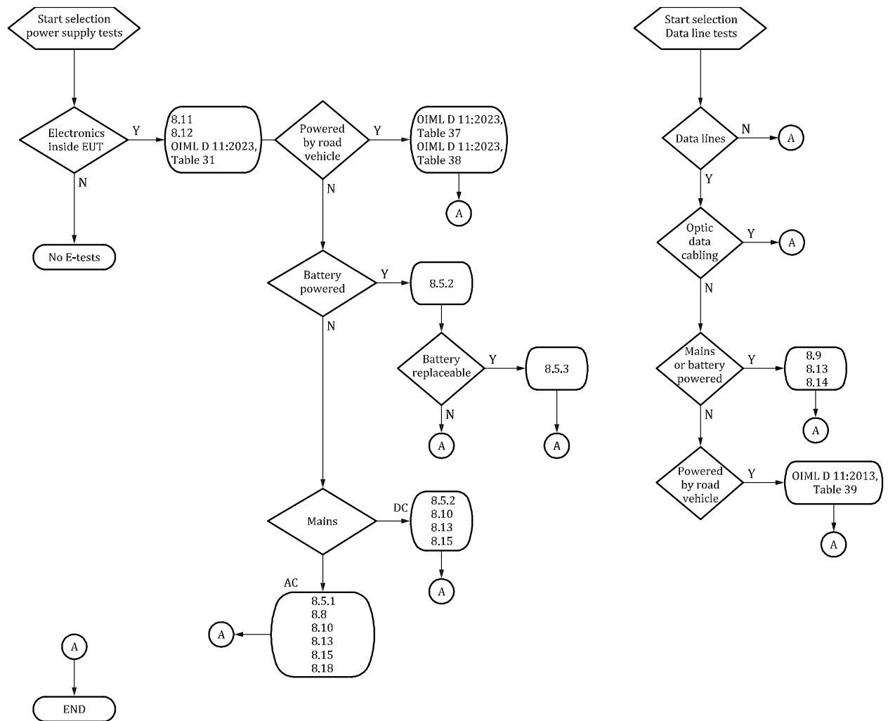
Figure 3 — Flow chart to determine the tests required in 8.5 and 8.8 to 8.15. Some test refer to OIML D 11:2013 [31]
