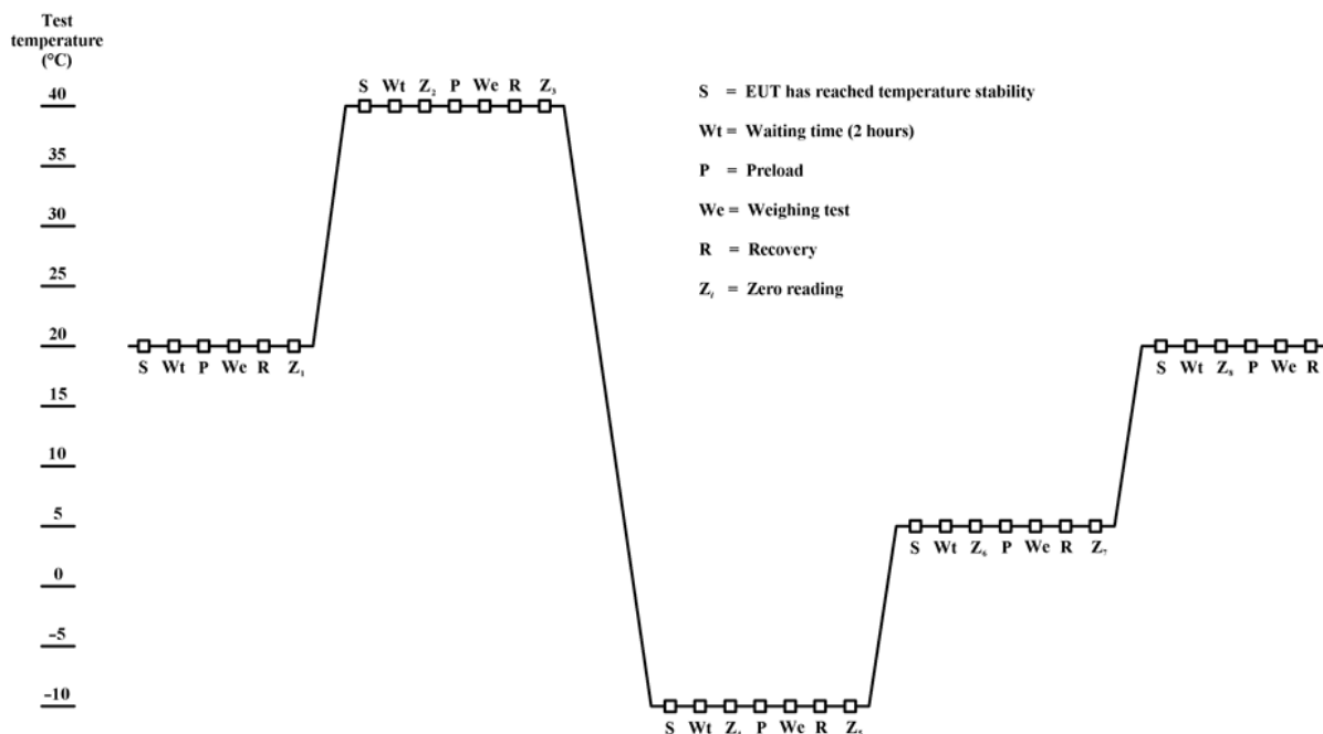
Figure 1 – Proposed test sequence for tests in 7.2.1 combined with 7.2.2 (temperature test where the temperature limits are –10 °C to +40 °C)
