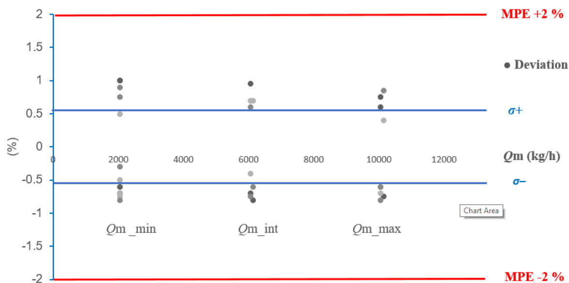
Figure 2 – Dispersion of results for totalisations of \Sigma_{\min}
