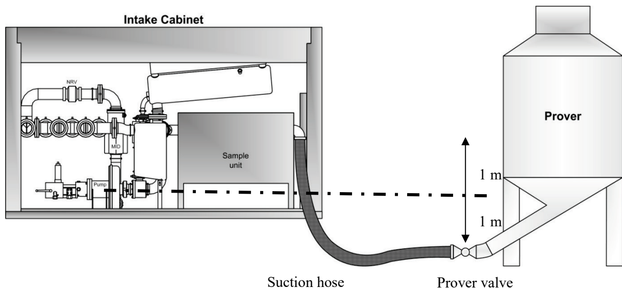
Test installation
