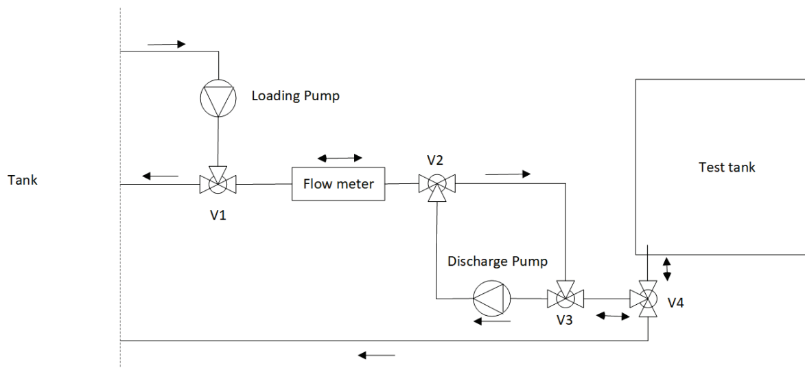
Figure X.K.1 Example of test rig for X.K.3 testing
